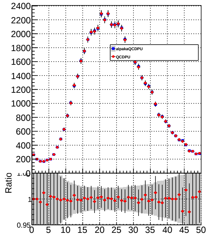
chargedHadronMultiplicity
