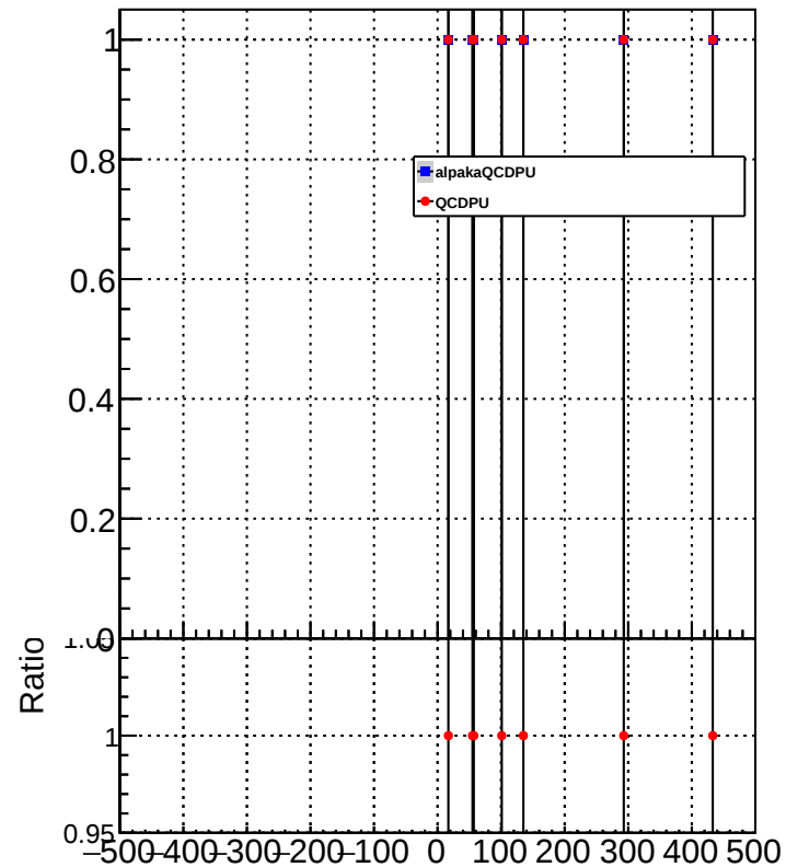
METResolution_GenMETTrue_MET500
