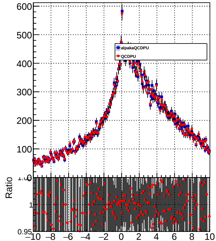
METUnc_JetResDown
