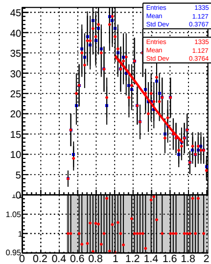
Jet response (pT/pTgen) in 15 \leq p_t < 21 , 2.5 \leq |\eta| < 3.0
