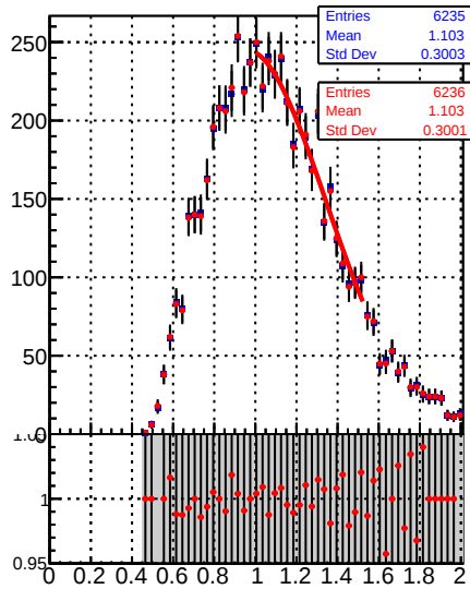
Jet response (pT/pTgen) in 15 \leq p_t < 21 , 0.5 \leq |\eta| < 1.3
