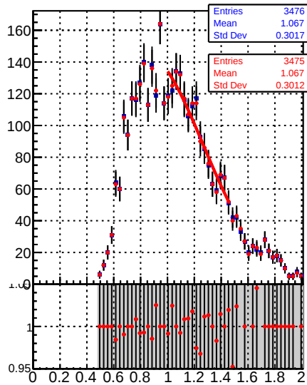
Jet response (pT/pTgen) in 15 \leq p_t < 21 , 3.0 \leq |\eta| < 5.0
