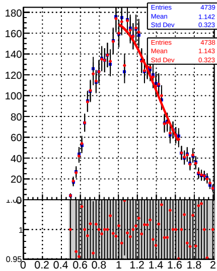
Jet response (pT/pTgen) in 15 \leq p_t < 21 , 1.3 \leq |\eta| < 2.1
