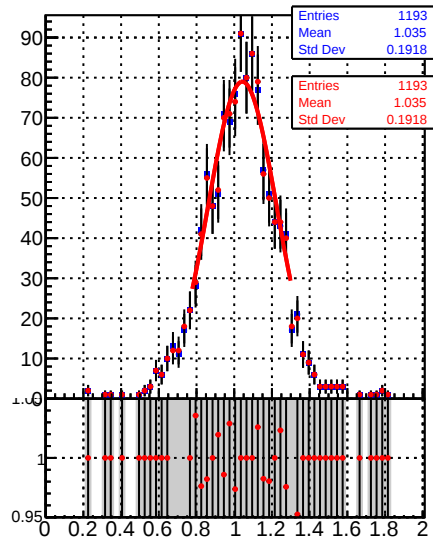
Jet response (pT/pTgen) in 64 <= pt < 84, 2.1 <= |eta| < 2.5
