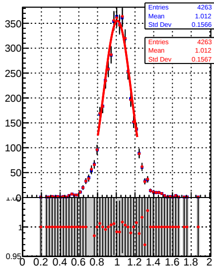
Jet response (pT/pTgen) in 64 <= pt < 84, 0.5 <= |eta| < 1.3
