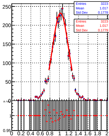
Jet response (pT/pTgen) in 64 <= pt < 84, 1.3 <= |eta| < 2.1
