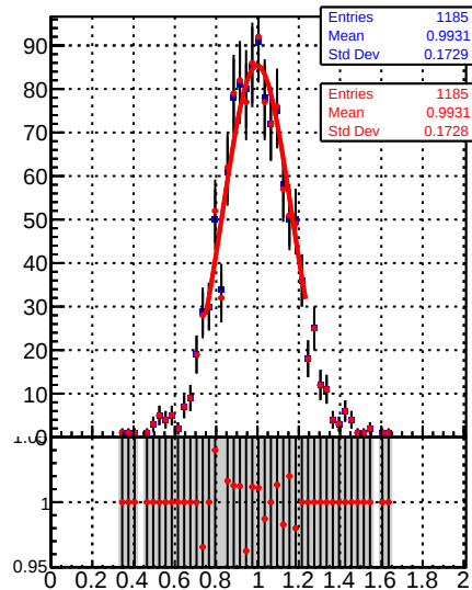
Jet response (pT/pTgen) in 64 <= pt < 84, 3.0 <= |eta| < 5.0
