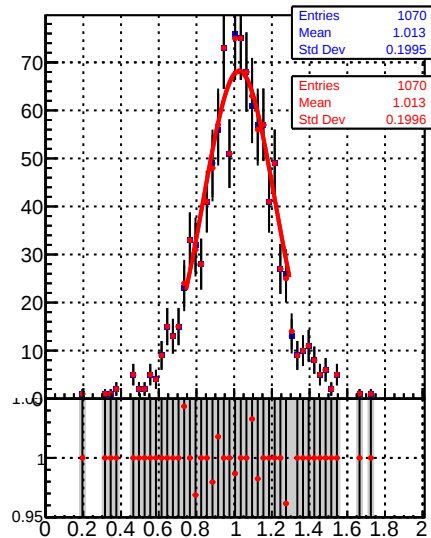
Jet response (pT/pTgen) in 64 <= pt < 84, 2.5 <= |eta| < 3.0
