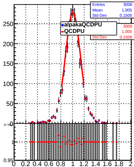
Jet response (pT/pTgen) in 64 <= pt < 84, 0.0 <= |eta| < 0.5
