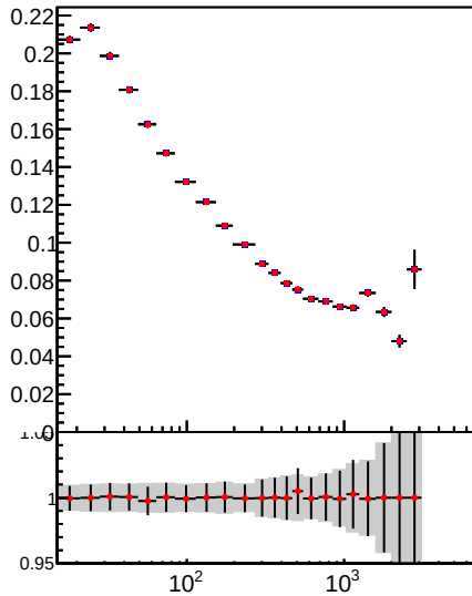
Raw Jet pT resolution using RMS, 0.5 < |\eta| < 1.3
