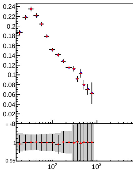
Raw Jet pT resolution using RMS, 2.5 < |\eta| < 3.0
