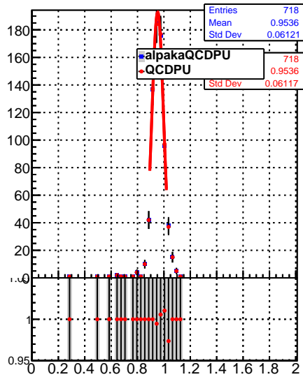
Raw Jet response (pT/pTgen) in 1032 &lt;math&gt;\leq p_t &lt; 1248, 0.0 \leq |\eta| &lt; 0.5&lt;/math&gt;
