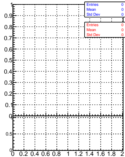
Raw Jet response (pT/pTgen) in 1032 &lt;math&gt;\leq p_t &lt; 1248, 2.5 \leq |\eta| &lt; 3.0&lt;/math&gt;
