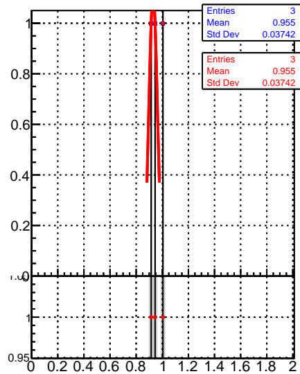
Raw Jet response (pT/pTgen) in 1032 &lt;math&gt;\leq p_t &lt; 1248, 2.1 \leq |\eta| &lt; 2.5&lt;/math&gt;
