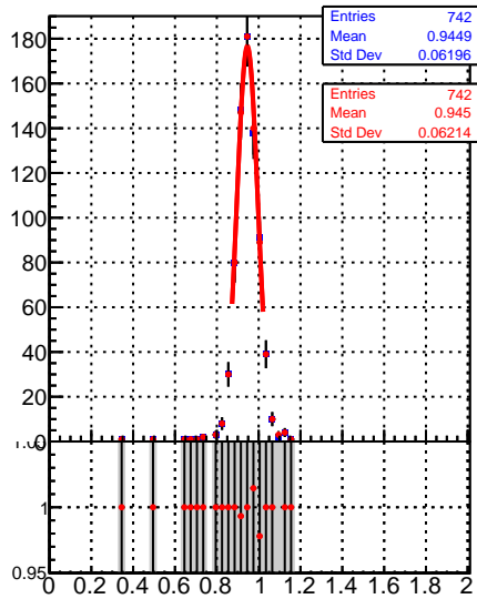
Raw Jet response (pT/pTgen) in 1032 &lt;math&gt;\leq p_t &lt; 1248, 0.5 \leq |\eta| &lt; 1.3&lt;/math&gt;
