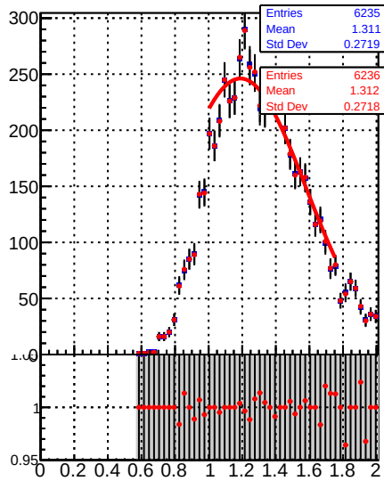
Raw Jet response (pT/pTgen) in 15 \leq pt < 21, 0.5 \leq |\eta| < 1.3
