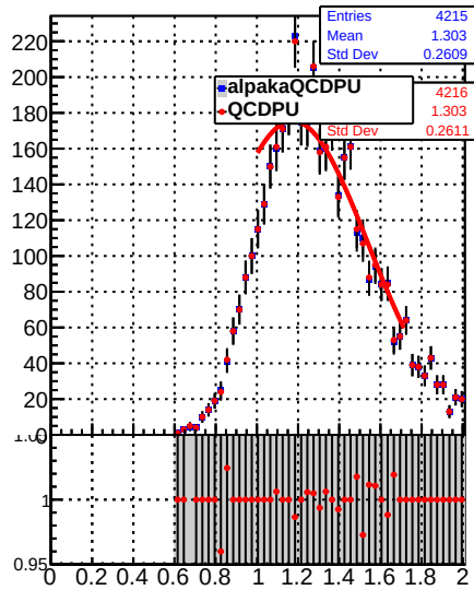
Raw Jet response (pT/pTgen) in 15 \leq pt < 21, 0.0 \leq |\eta| < 2.1
