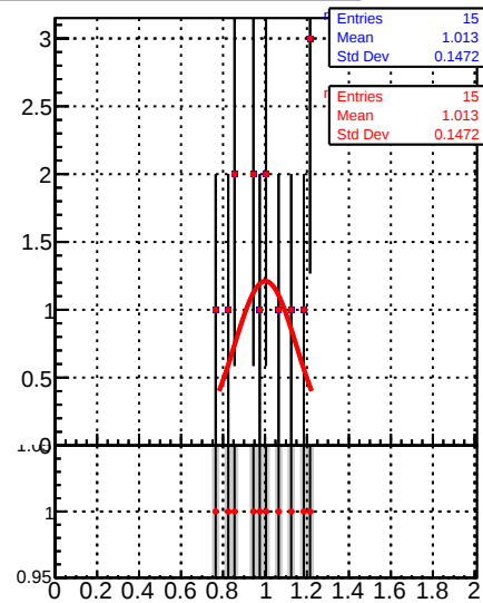
Raw Jet response (pT/pTgen) in 330 &lt;= pt &lt; 395, 3.0 &lt;= [eta] &lt; 5.0
