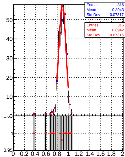
Raw Jet response (pT/pTgen) in 330 &lt;= pt &lt; 395, 2.1 &lt;= [eta] &lt; 2.5
