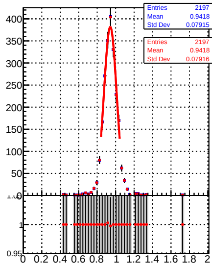
Raw Jet response (pT/pTgen) in 330 &lt;= pt &lt; 395, 0.5 &lt;= [eta] &lt; 1.3
