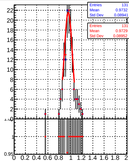
Raw Jet response (pT/pTgen) in 330 &lt;= pt &lt; 395, 2.5 &lt;= [eta] &lt; 3.0
