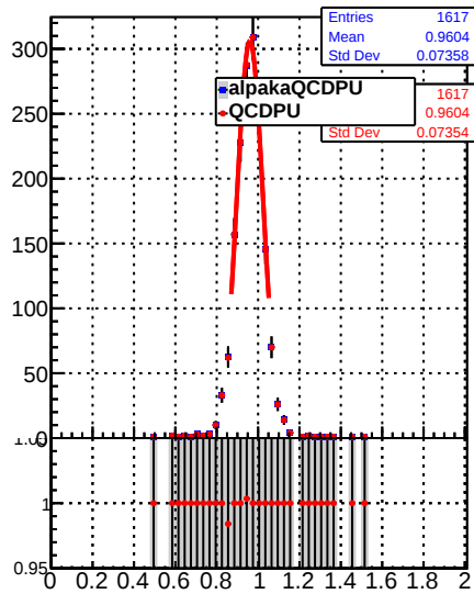
Raw Jet response (pT/pTgen) in 330 &lt;= pt &lt; 395, 0.0 &lt;= [eta] &lt; 0.5
