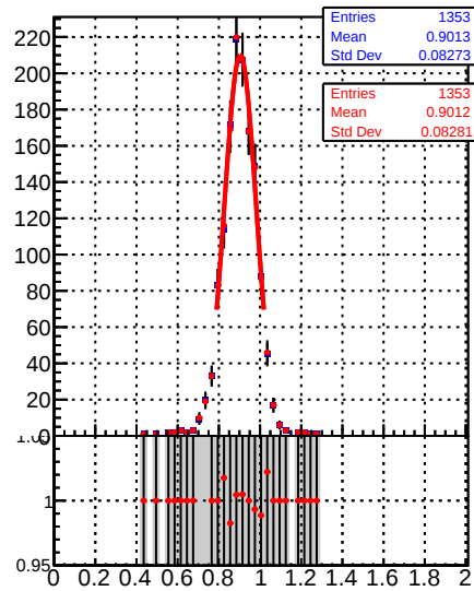
Raw Jet response (pT/pTgen) in 330 &lt;= pt &lt; 395, 1.3 &lt;= [eta] &lt; 2.1
