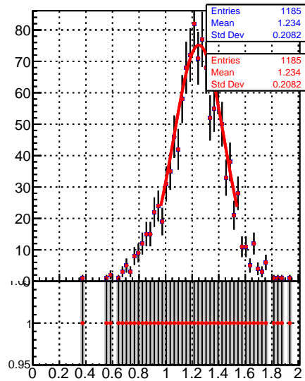
Raw Jet response (pT/pTgen) in 64 &lt;= pt &lt; 84, 3.0 &lt;= |eta| &lt; 5.0
