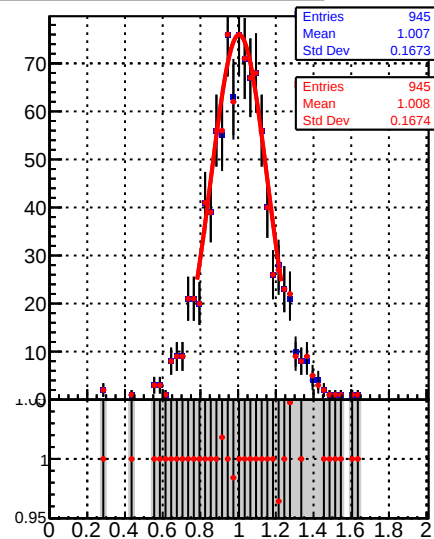
Jet response (pT/pTgen) in 84 <= pt < 114, 3.0 <= |eta| < 5.0
