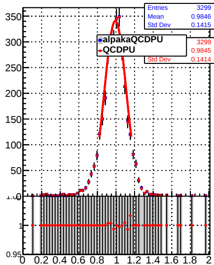
Jet response (pT/pTgen) in 84 <= pt < 114, 0.0 <= |eta| < 0.5
