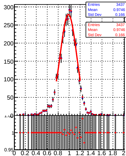
Jet response (pT/pTgen) in 84 <= pt < 114, 1.3 <= |eta| < 2.1
