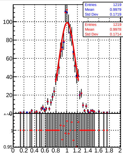
Jet response (pT/pTgen) in 84 <= pt < 114, 2.1 <= |eta| < 2.5
