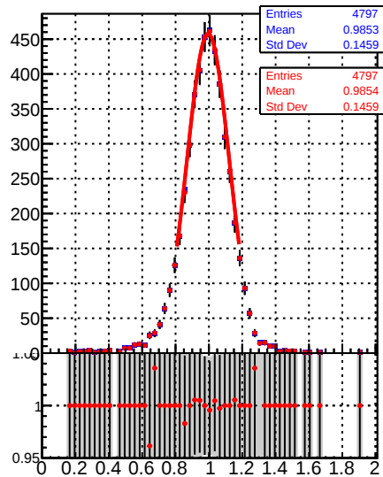
Jet response (pT/pTgen) in 84 <= pt < 114, 0.5 <= |eta| < 1.3
