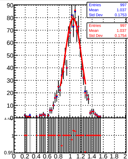
Jet response (pT/pTgen) in 84 <= pt < 114, 2.5 <= |eta| < 3.0
