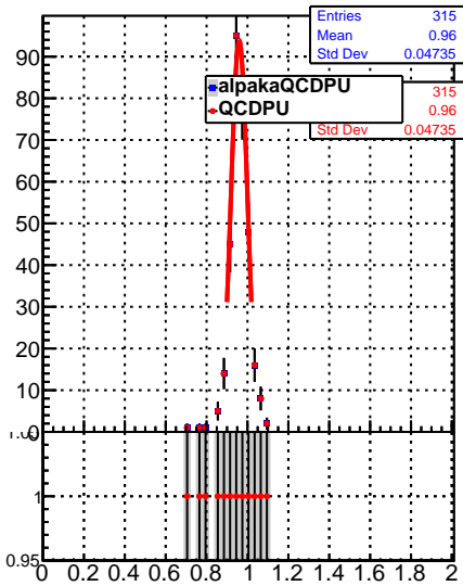
Raw Jet response (pT/pTgen) in 1588 &lt;math&gt;\leq p_t &lt; 2000, 0.0 \leq |\eta| &lt; 0.5&lt;/math&gt;
