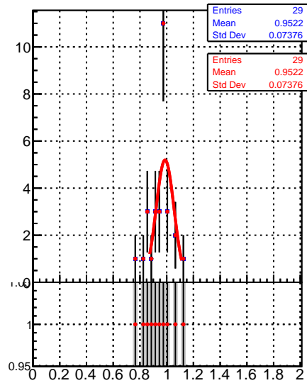
Raw Jet response (pT/pTgen) in 1588 &lt;math&gt;\leq p_t &lt; 2000, 1.3 \leq |\eta| &lt; 2.1&lt;/math&gt;
