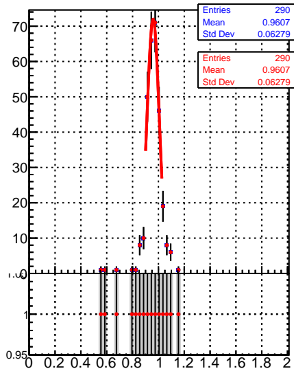
Raw Jet response (pT/pTgen) in 1588 &lt;math&gt;\leq p_t &lt; 2000, 0.5 \leq |\eta| &lt; 1.3&lt;/math&gt;
