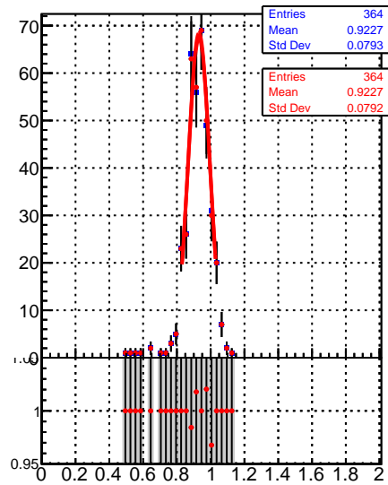
Raw Jet response (pT/pTgen) in 846 &lt;= pt &lt; 1032, 1.3 &lt;= |eta| &lt; 2.1
