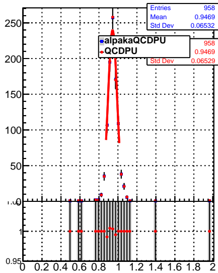
Raw Jet response (pT/pTgen) in 846 &lt;= pt &lt; 1032, 0.0 &lt;= |eta| &lt; 0.5
