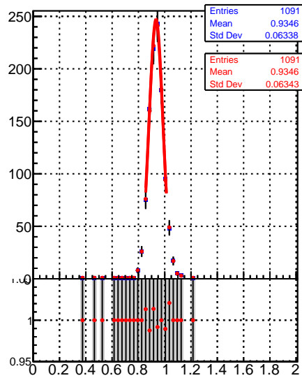
Raw Jet response (pT/pTgen) in 846 &lt;= pt &lt; 1032, 0.5 &lt;= |eta| &lt; 1.3
