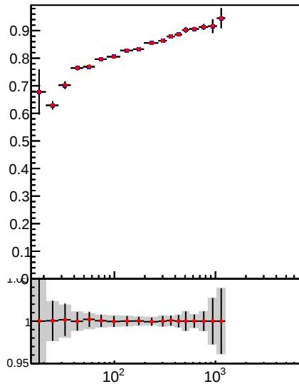
Raw Jet pT response, 2.1 < |\eta| < 2.5
