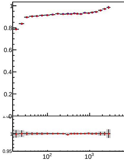
Raw Jet pT response, 0.5 < |\eta| < 1.3
