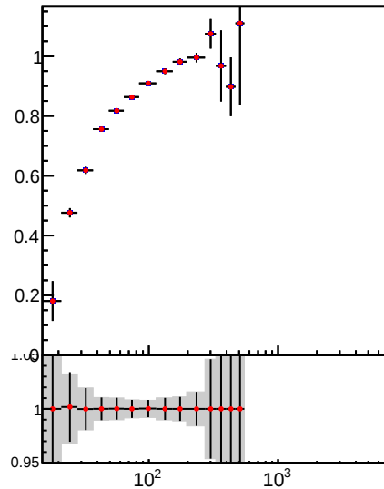
Raw Jet pT response, 3.0 < |\eta| < 5.0
