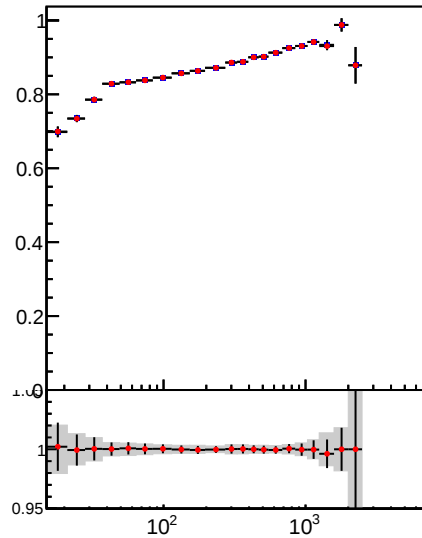
Raw Jet pT response, 1.3 < |\eta| < 2.1
