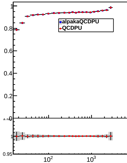
Raw Jet pT response, 0.0 < |\eta| < 0.5
