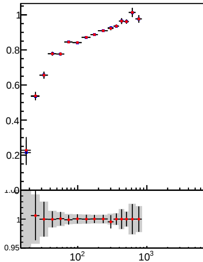
Raw Jet pT response, 2.5 < |\eta| < 3.0
