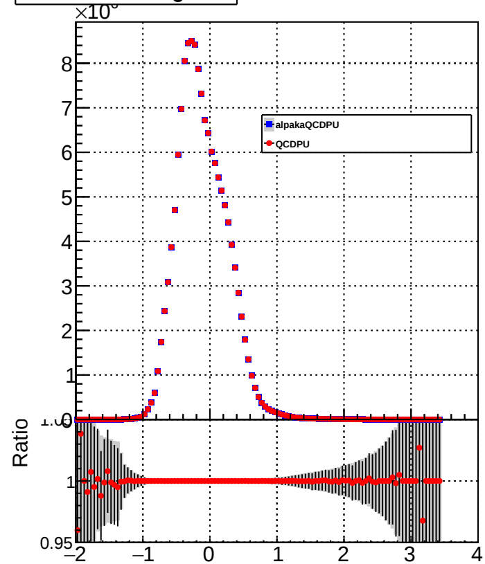
AllCandidateLog10Pt
