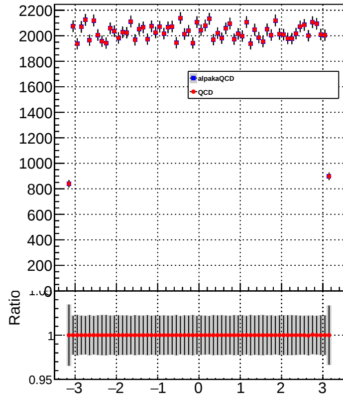
CorrJetPhi Pt>40
