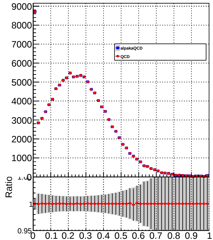
photonEnergyFraction
