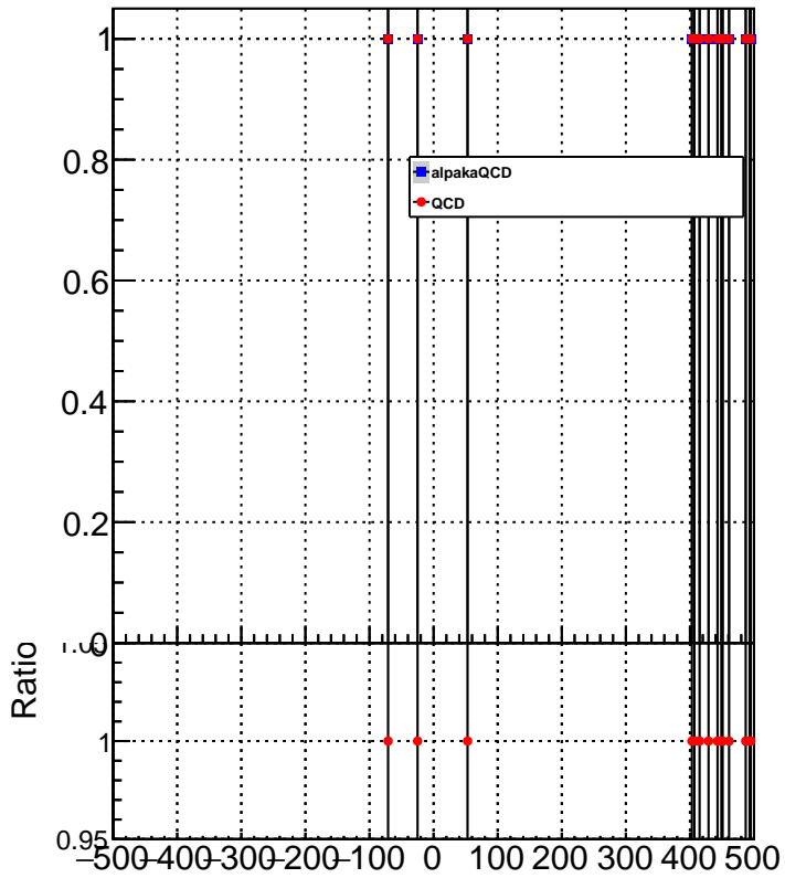
METResolution_GenMETTrue_MET400to500
