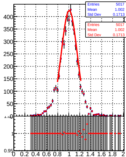
Jet response ( p_T/p_{T\text{gen}} ) in 28 \leq p_t < 37, 0.5 \leq |\eta| < 1.3
