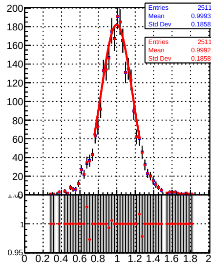
Jet response ( p_T/p_{T\text{gen}} ) in 28 \leq p_t < 37, 3.0 \leq |\eta| < 5.0
