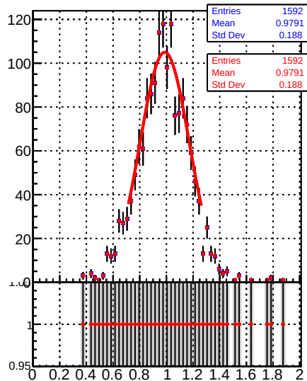
Jet response ( p_T/p_{T\text{gen}} ) in 28 \leq p_t < 37, 2.1 \leq |\eta| < 2.5
