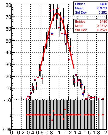
Jet response ( p_T/p_{T\text{gen}} ) in 28 \leq p_t < 37, 2.5 \leq |\eta| < 3.0
