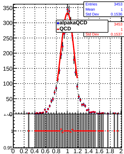
Jet response ( p_T/p_{T\text{gen}} ) in 28 \leq p_t < 37, 0.0 \leq |\eta| < 0.5
