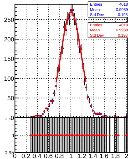
Jet response ( p_T/p_{T\text{gen}} ) in 28 \leq p_t < 37, 1.3 \leq |\eta| < 2.1
