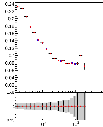
Jet pT resolution using RMS, 1.3 < |\eta| < 2.1
