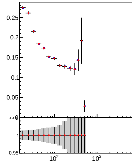
Jet pT resolution using RMS, 3.0 < |\eta| < 5.0
