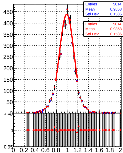
Jet response (pT/pTgen) in 37 \leq p_t < 49, 0.5 \leq |\eta| < 1.3
