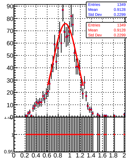
Jet response (pT/pTgen) in 37 \leq p_t < 49, 2.5 \leq |\eta| < 3.0
