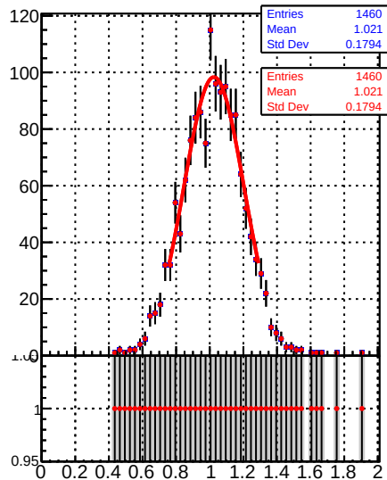
Jet response (pT/pTgen) in 37 \leq p_t < 49, 2.1 \leq |\eta| < 2.5
