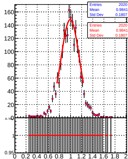
Jet response (pT/pTgen) in 37 \leq p_t < 49, 3.0 \leq |\eta| < 5.0
