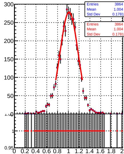
Jet response (pT/pTgen) in 37 \leq p_t < 49, 1.3 \leq |\eta| < 2.1
