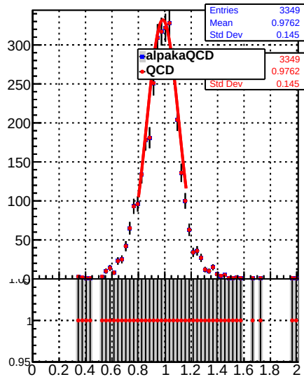
Jet response (pT/pTgen) in 37 \leq p_t < 49, 0.0 \leq |\eta| < 0.5
