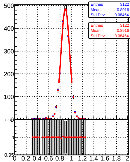
Raw Jet response (pT/pTgen) in 196 \leq p_t < 272 , 1.3 \leq |\eta| < 2.1
