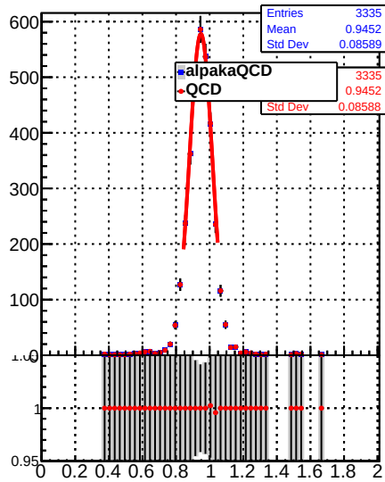
Raw Jet response (pT/pTgen) in 196 \leq p_t < 272 , 0.0 \leq |\eta| < 0.5
