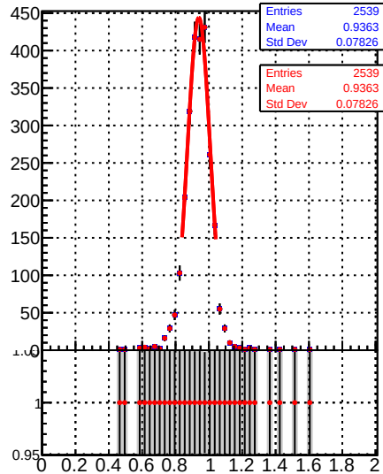
Raw Jet response (pT/pTgen) in 272 \leq p_t < 330 , 0.5 \leq |\eta| < 1.3
