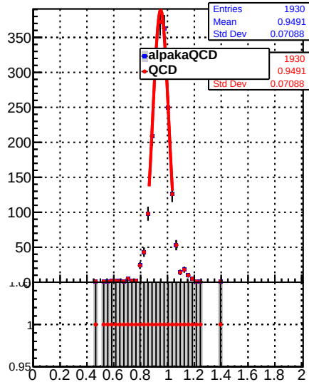
Raw Jet response (pT/pTgen) in 272 \leq p_t < 330 , 0.0 \leq |\eta| < 2.5
