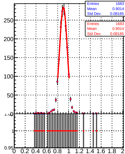
Raw Jet response (pT/pTgen) in 272 \leq p_t < 330 , 1.3 \leq |\eta| < 2.1
