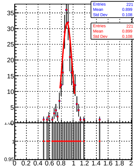
Raw Jet response (pT/pTgen) in 272 \leq p_t < 330 , 2.5 \leq |\eta| < 3.0
