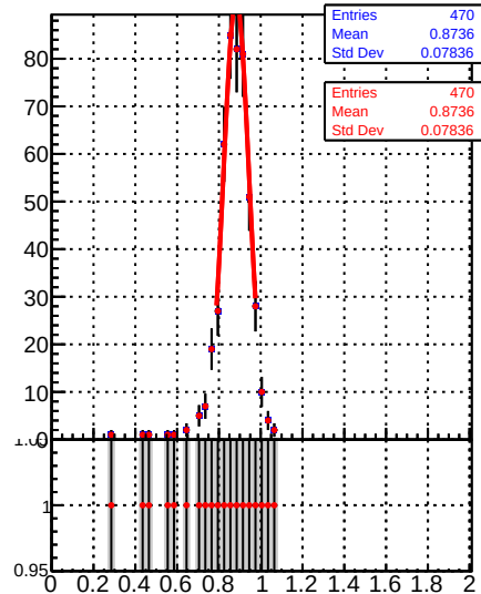
Raw Jet response (pT/pTgen) in 272 \leq p_t < 330 , 2.1 \leq |\eta| < 2.5
