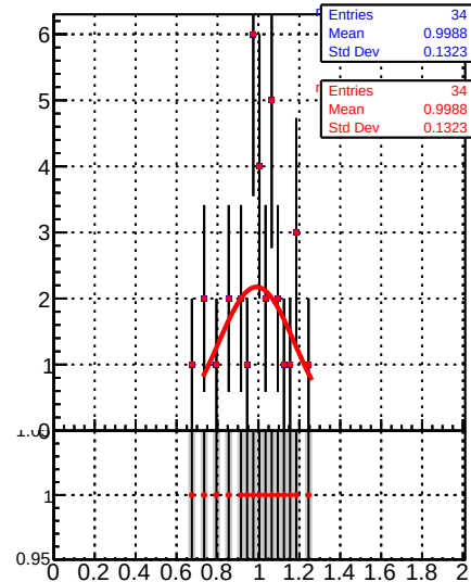
Raw Jet response (pT/pTgen) in 272 \leq p_t < 330 , 3.0 \leq |\eta| < 5.0
