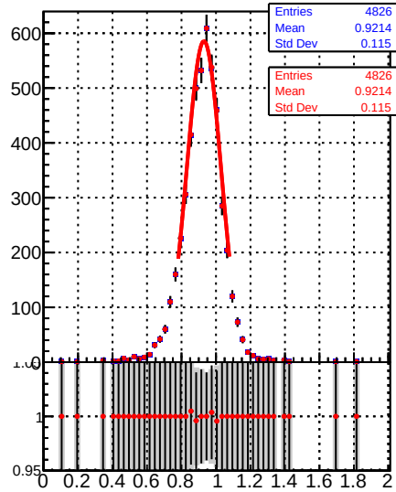
Raw Jet response (pT/pTgen) in 84 \leq pt < 114, 0.5 \leq |\eta| < 1.3
