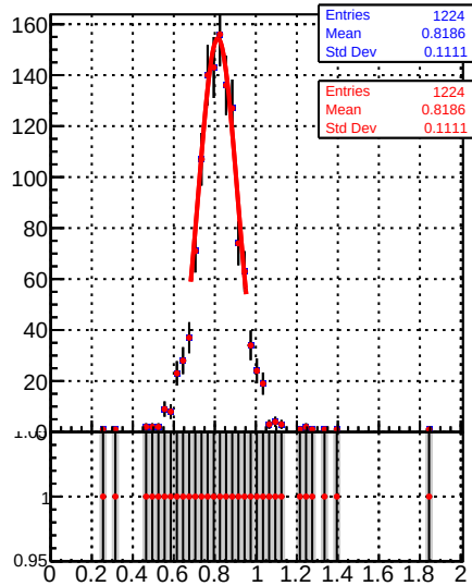
Raw Jet response (pT/pTgen) in 84 \leq pt < 114, 2.1 \leq |\eta| < 2.5
