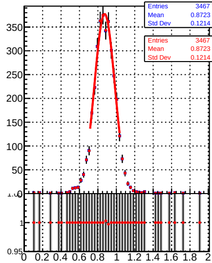
Raw Jet response (pT/pTgen) in 84 \leq pt < 114, 1.3 \leq |\eta| < 2.1
