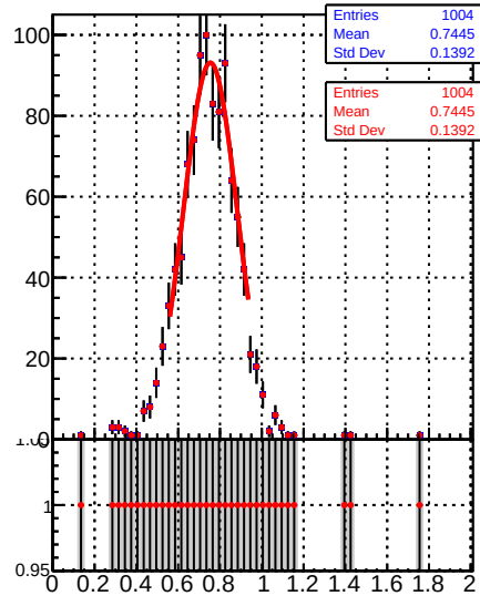
Raw Jet response (pT/pTgen) in 84 \leq pt < 114, 2.5 \leq |\eta| < 3.0
