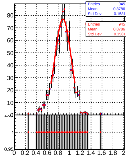
Raw Jet response (pT/pTgen) in 84 \leq pt < 114, 3.0 \leq |\eta| < 5.0
