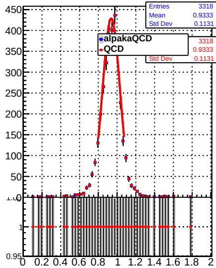
Raw Jet response (pT/pTgen) in 84 \leq pt < 114, 0.0 \leq |\eta| < 0.5
