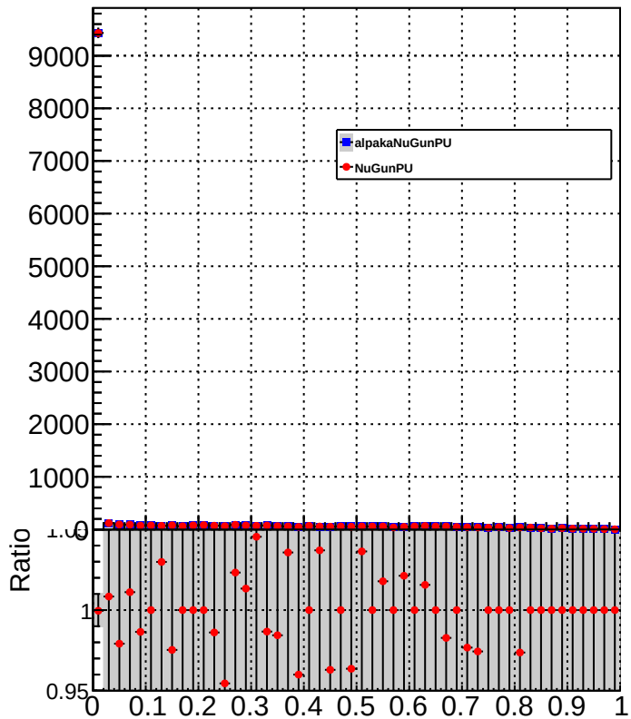
chargedHadronEnergyFraction
