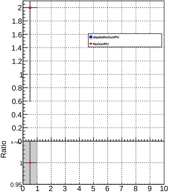
electronMultiplicity
