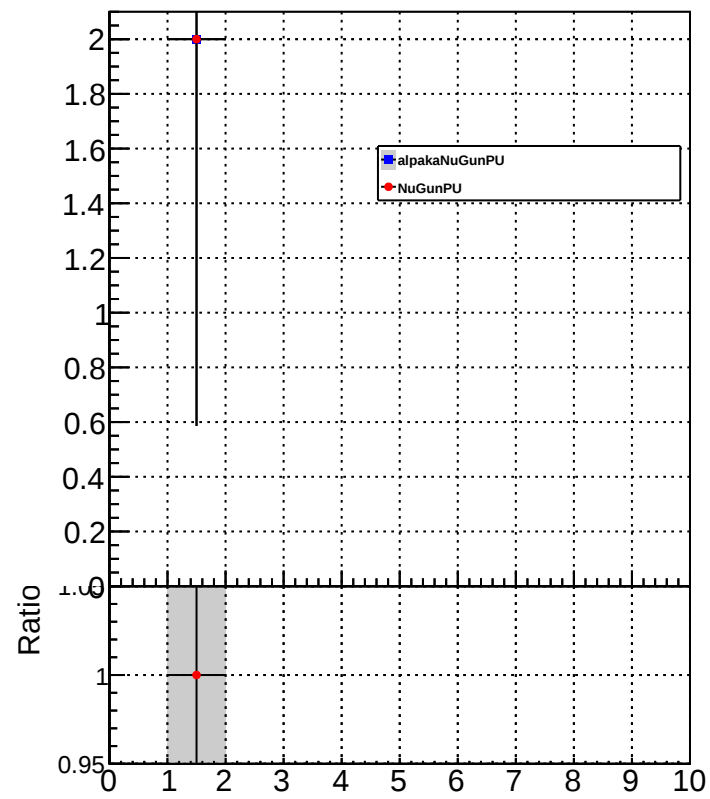
muonMultiplicity
