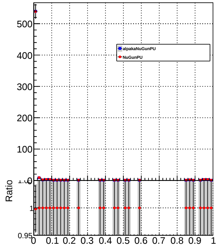
chargedMuEnergyFraction
