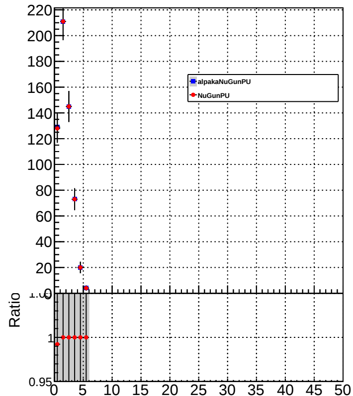
neutralHadronMultiplicity
