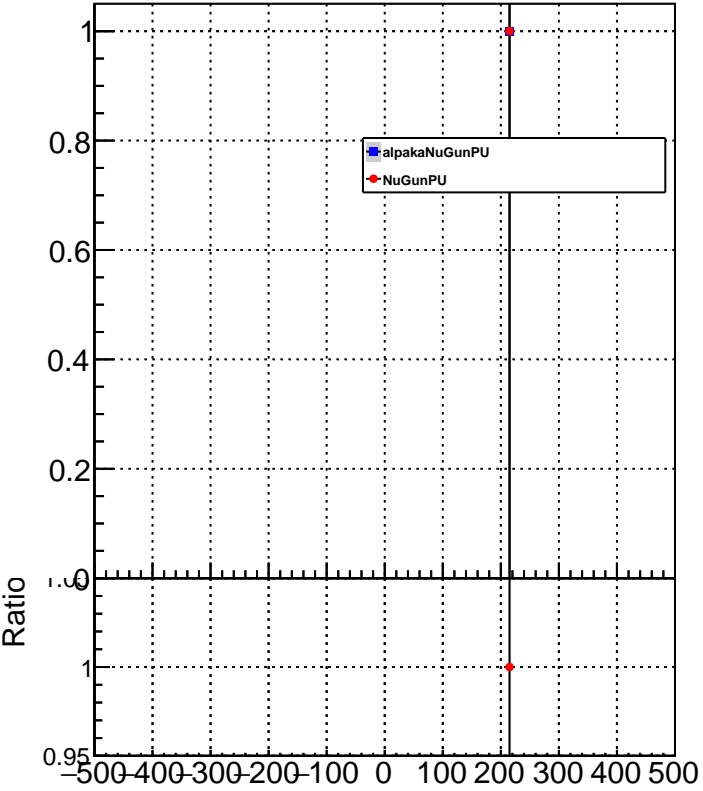
METResolution_GenMETTrue_MET200to300
