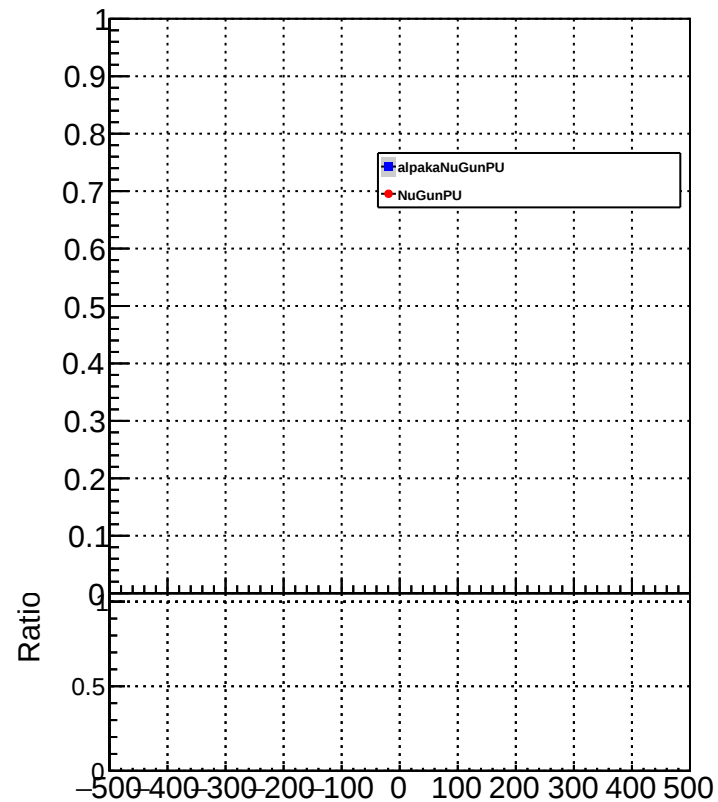
METResolution_GenMETTrue_MET300to400
