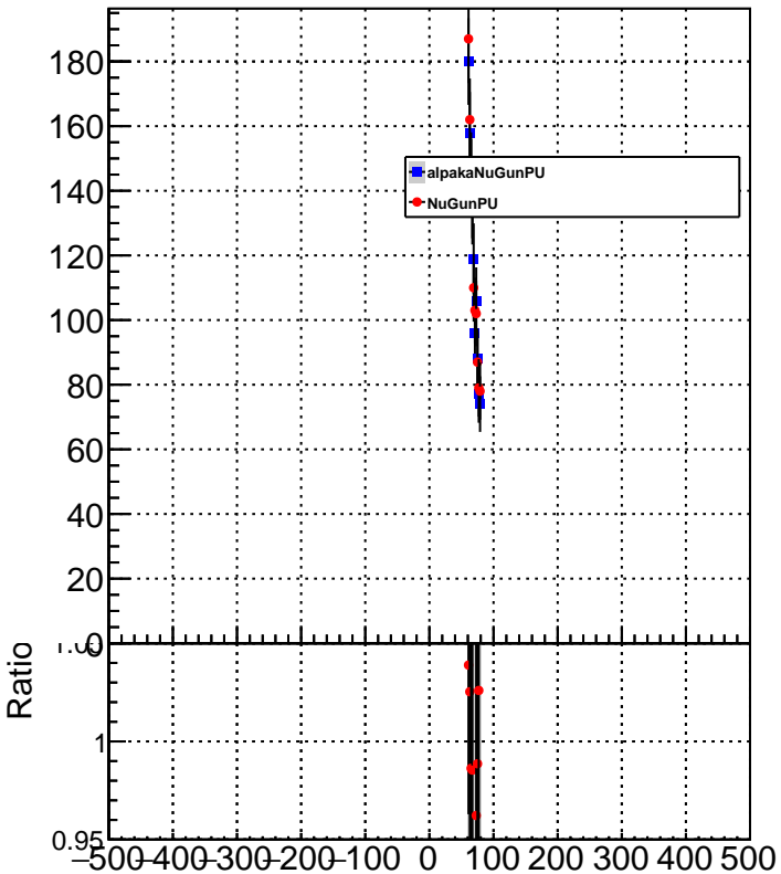
METResolution_GenMETTrue_MET60to80
