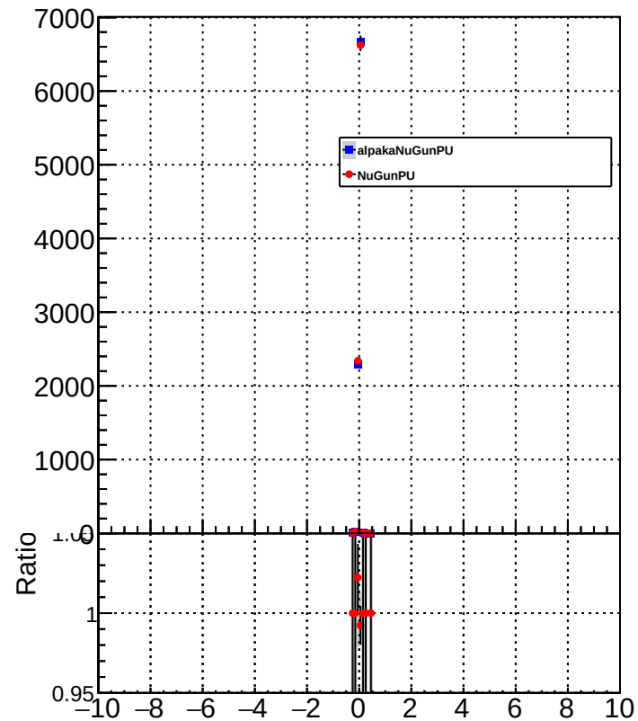
METUnc_ElectronEnUp
