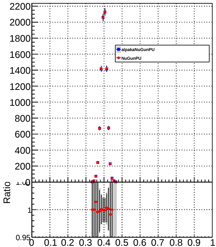
chargedHadronEtFraction
