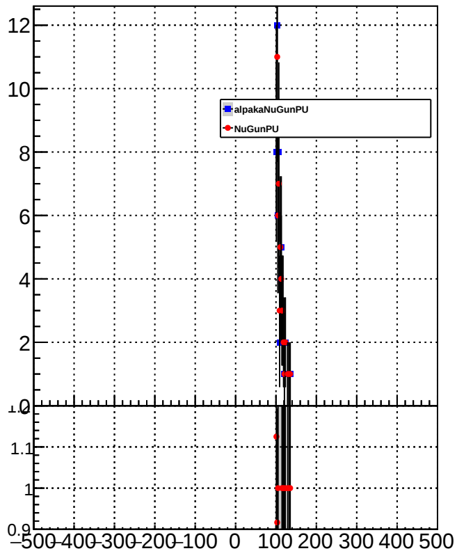
METResolution_GenMETTrue_MET100to150
