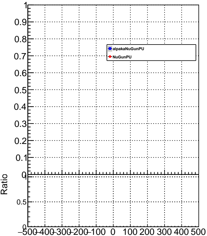
METResolution_GenMETTrue_MET300to400
