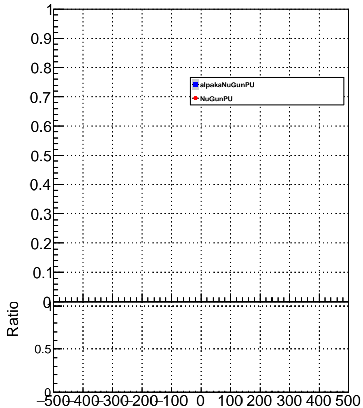
METResolution_GenMETTrue_MET500
