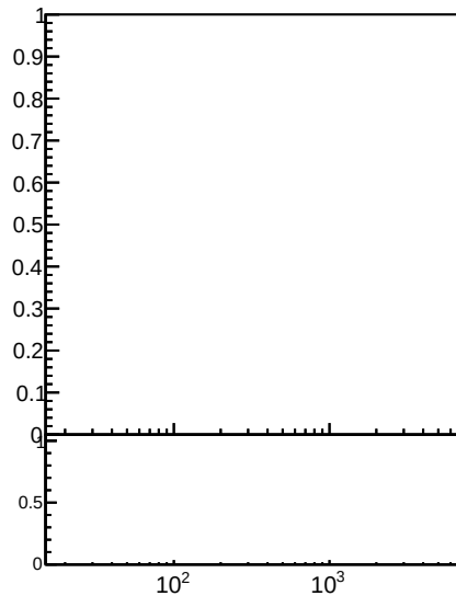
Raw Jet pT response, 2.5 < |\eta| < 3.0
