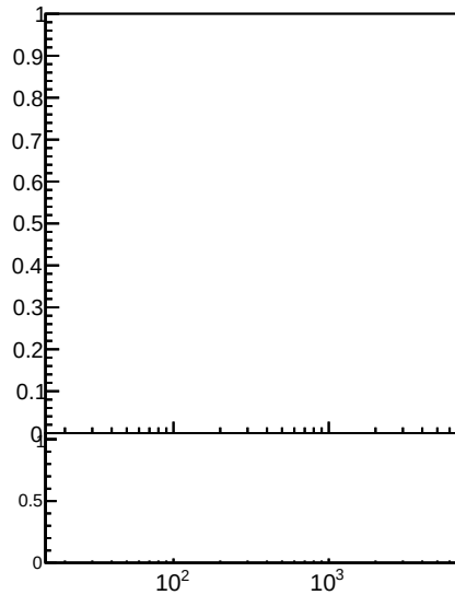
Raw Jet pT response, 0.5 < |\eta| < 1.3
