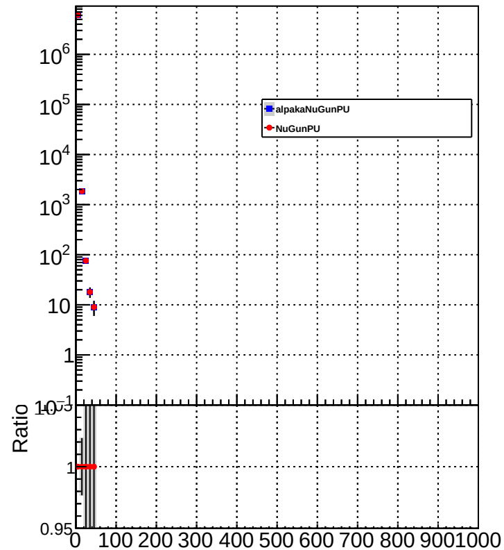
HF_hadronPtHigh
