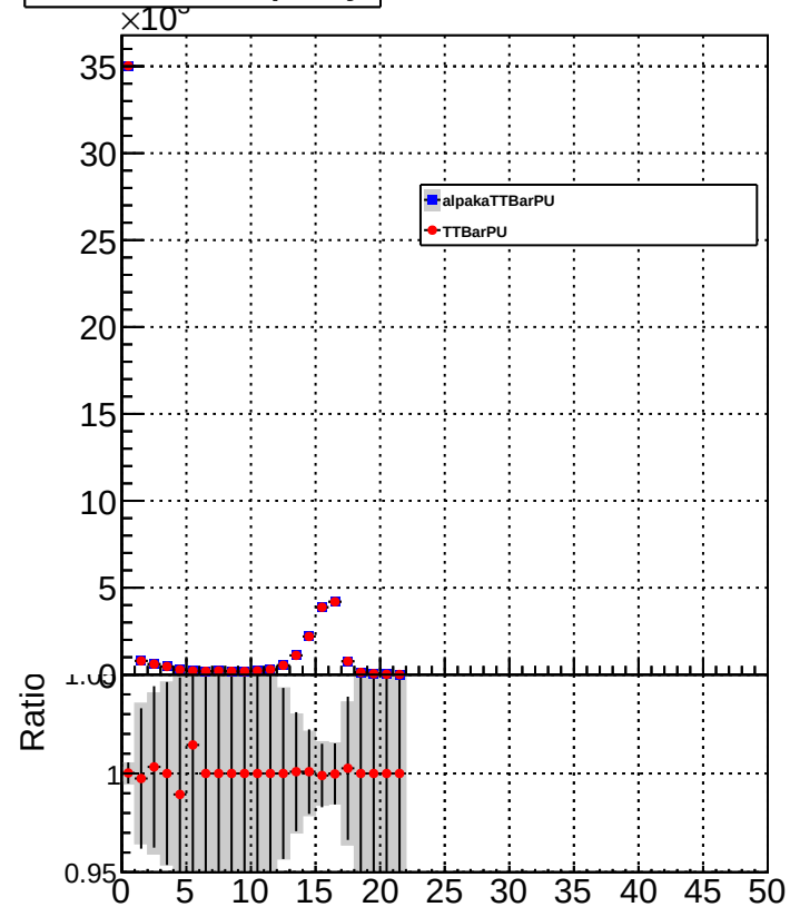
HFHadronMultiplicity
