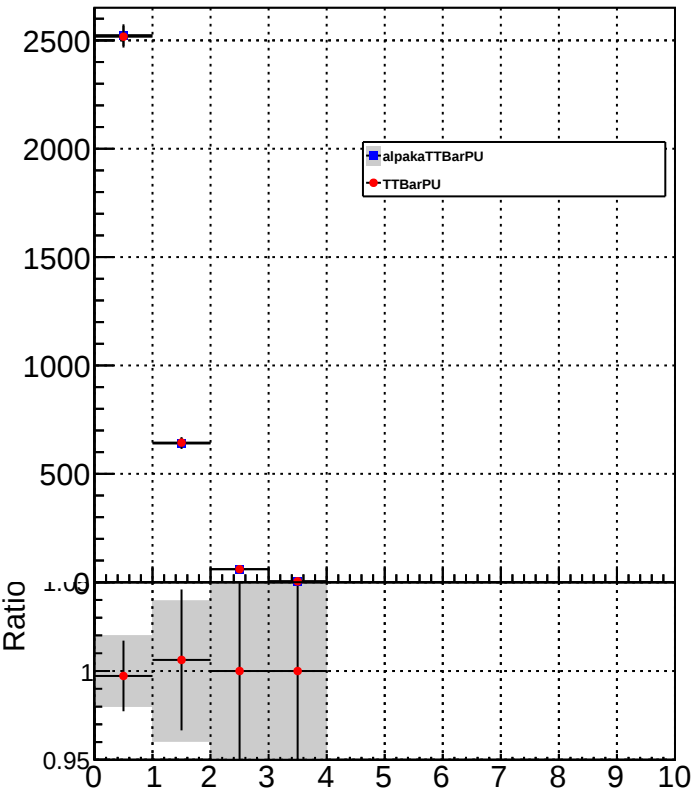
electronMultiplicity
