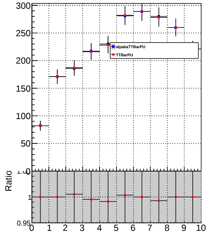
photonMultiplicity
