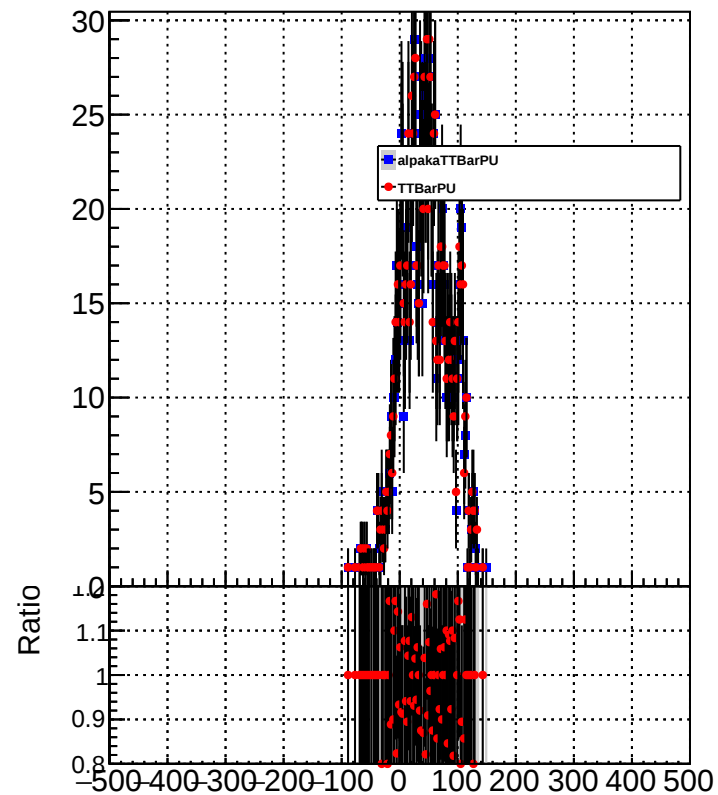
METResolution_GenMETTrue_MET100to150
