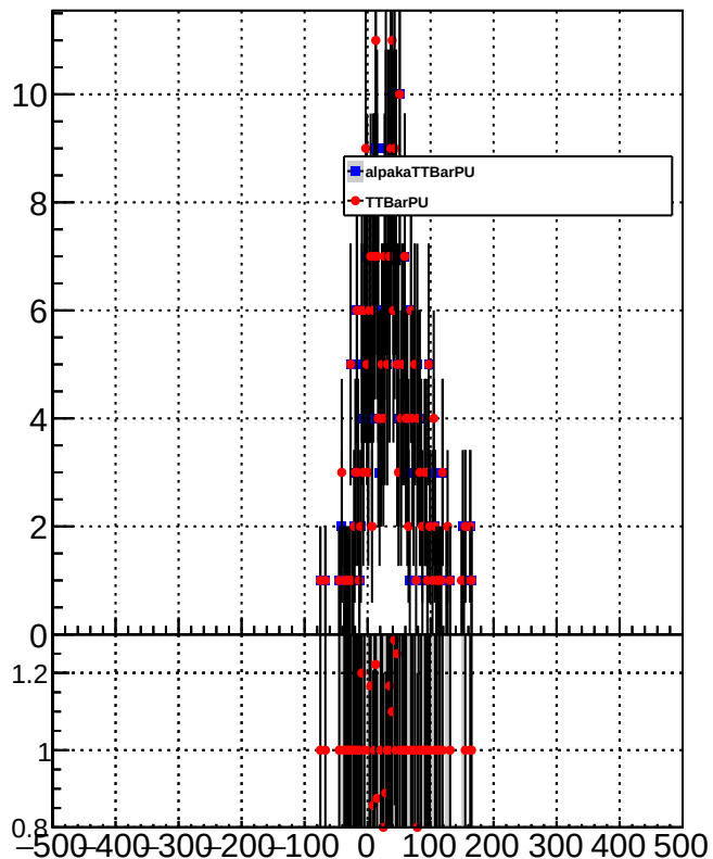
METResolution_GenMETTrue_MET150to200
