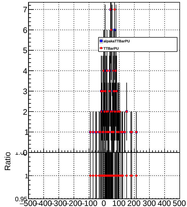
METResolution_GenMETTrue_MET200to300
