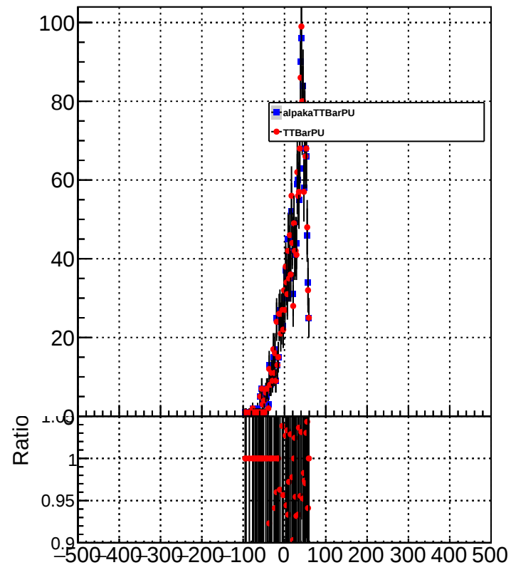
METResolution_GenMETTrue_MET40to60
