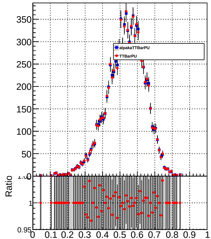
chargedHadronEtFraction
