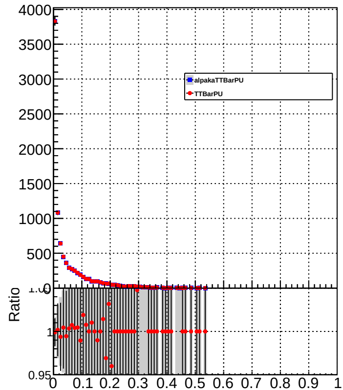
electronEtFraction
