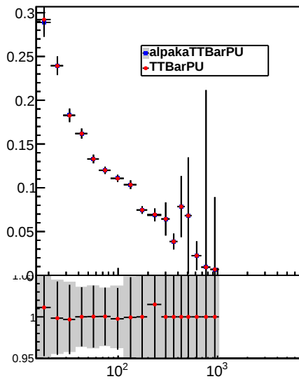
Jet pT resolution, 0.0 < |\eta| < 0.5
