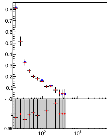
Jet pT resolution, 2.1 < |\eta| < 2.5
