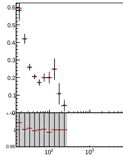
Jet pT resolution, 3.0 < |\eta| < 5.0
