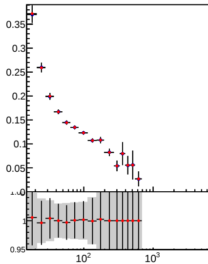
Jet pT resolution, 0.5 < |\eta| < 1.3
