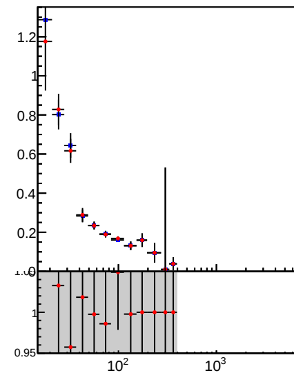
Jet pT resolution, 2.5 < |\eta| < 3.0
