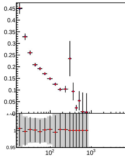
Jet pT resolution, 1.3 < |\eta| < 2.1
