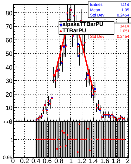
Jet response (pT/pTgen) in 21 \leq p_t < 28, 0.0 \leq |\eta| < 1.3
